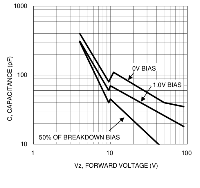
Fig.6 Typical Capacitance versus V_z
