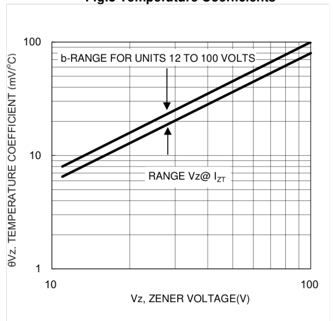
Fig.8 Temperature Coefficients
