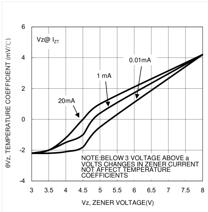
Fig.9 Effect Of Zener Current
