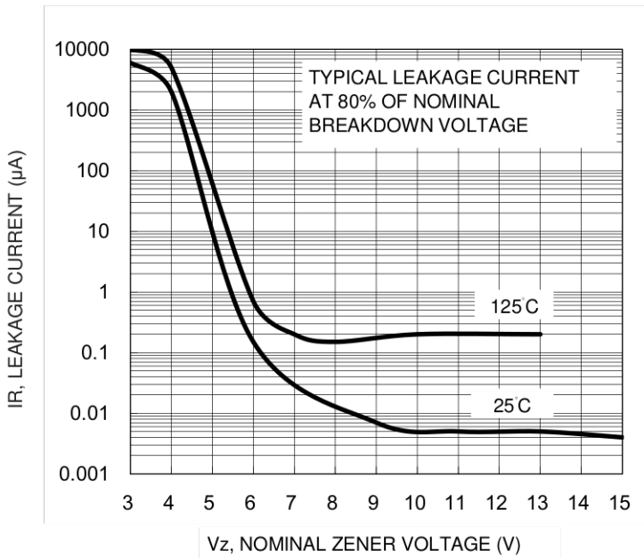
Fig.5 Typical Leakage Current
