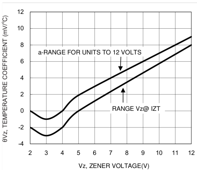
Fig.7 Temperature Coefficients
